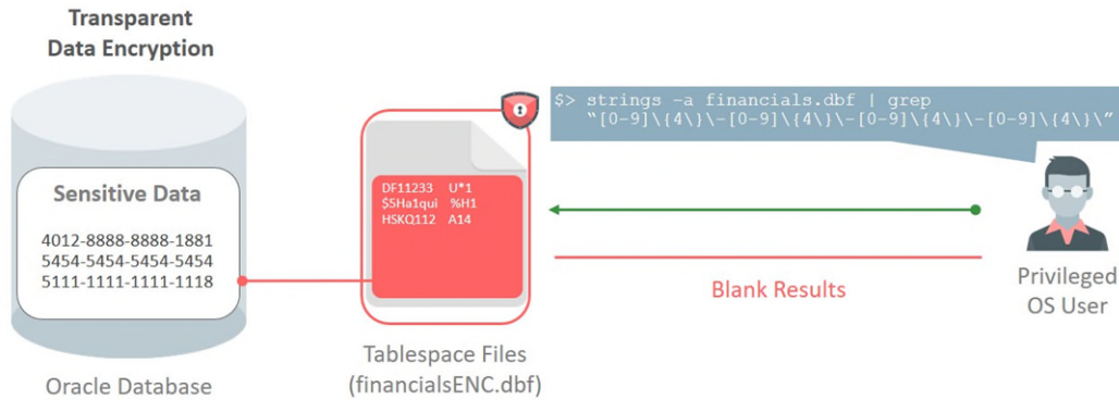
Figure 2. Encrypting with Transparent Data Encryption to prevent database bypass.
