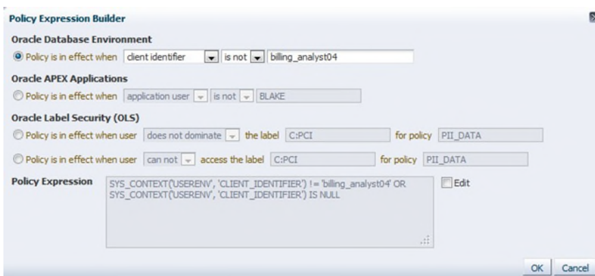
Figure 7. Using Oracle Enterprise Manager Policy Expression Builder to create Data Redaction policies
